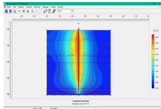
Gambar 4. Perpindahan Total
