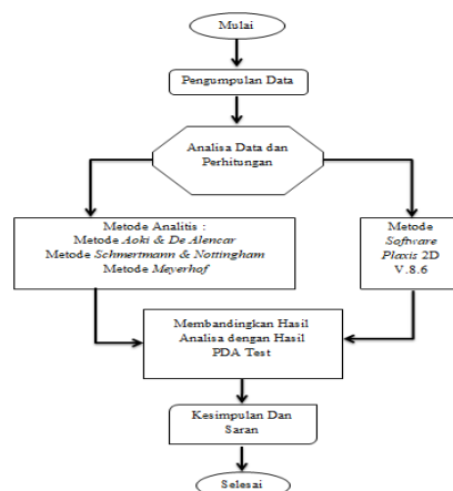
Gambar 2. Diagram Alir
