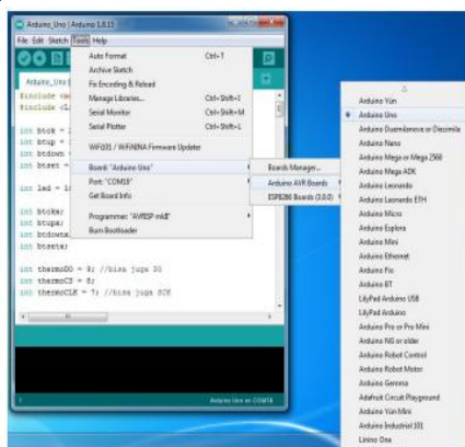
Figure 7. AU Board Settings Display
