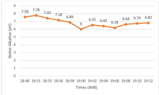
Figure 13. Water Alkaline Level Graph in the first test
