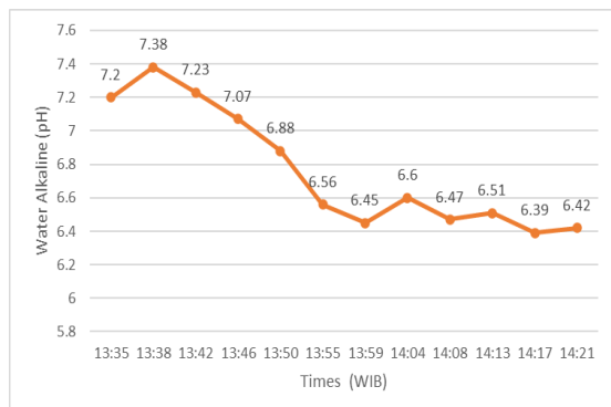
Figure 16. Graph of the Water Alkaline Level in the second test
