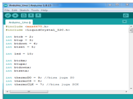
Figure 6. Sketch Arduino IDE
