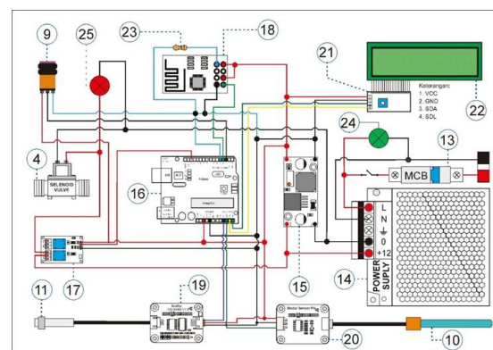
Figure 4. Overall Network Design
