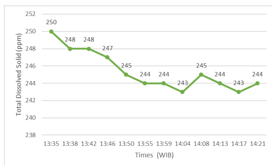
Figure 17. Total Dissolved Solid graph in the second test
