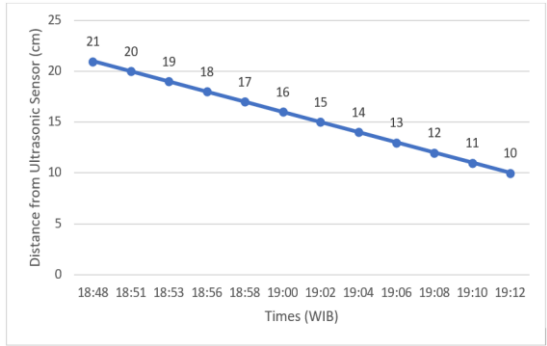
Figure 12. Graph of water distance from the Ultrasonic sensor in the first test
