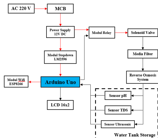
Figure 1. Hardware Design Block Diagram
