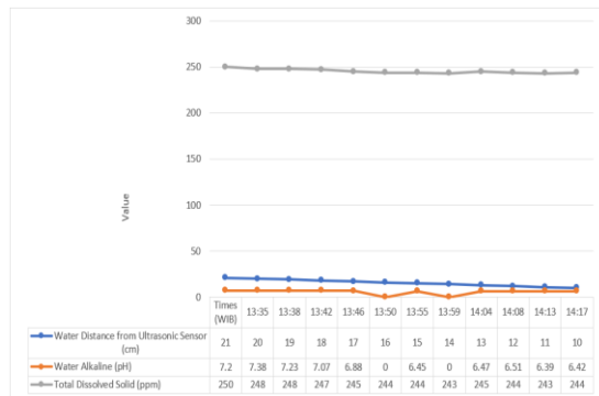
Figure 19 Performance Comparison Graph of Each Second Test Sensor
