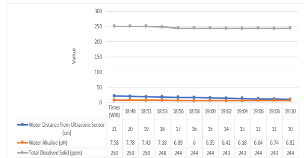
Figure 18 Performance Comparison Graph of Each First Test Sensor
