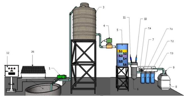
Figure 3. Brackish Water Desalination System
