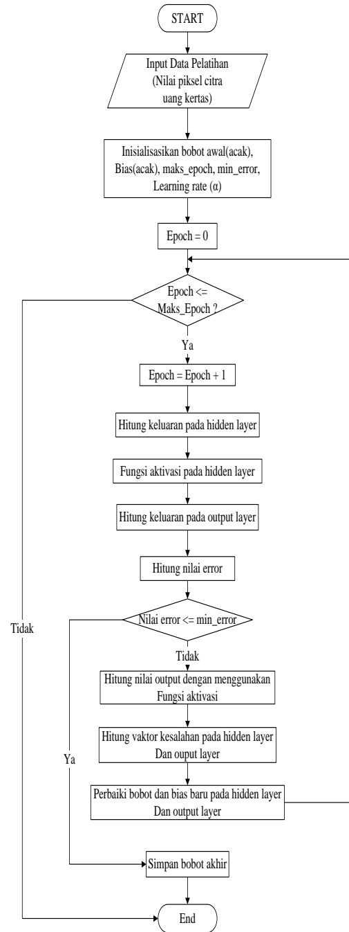
Gambar 7. Flowchart Pelatihan Backpropagation
