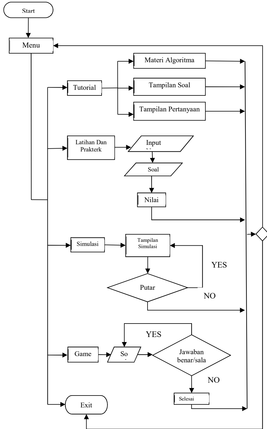
Gambar 1. Flowchart
