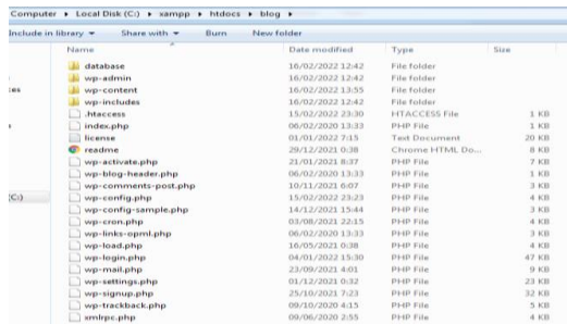
Gambar 2. File Wordpress
