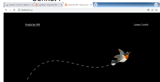
Gambar 6. Halaman Website
